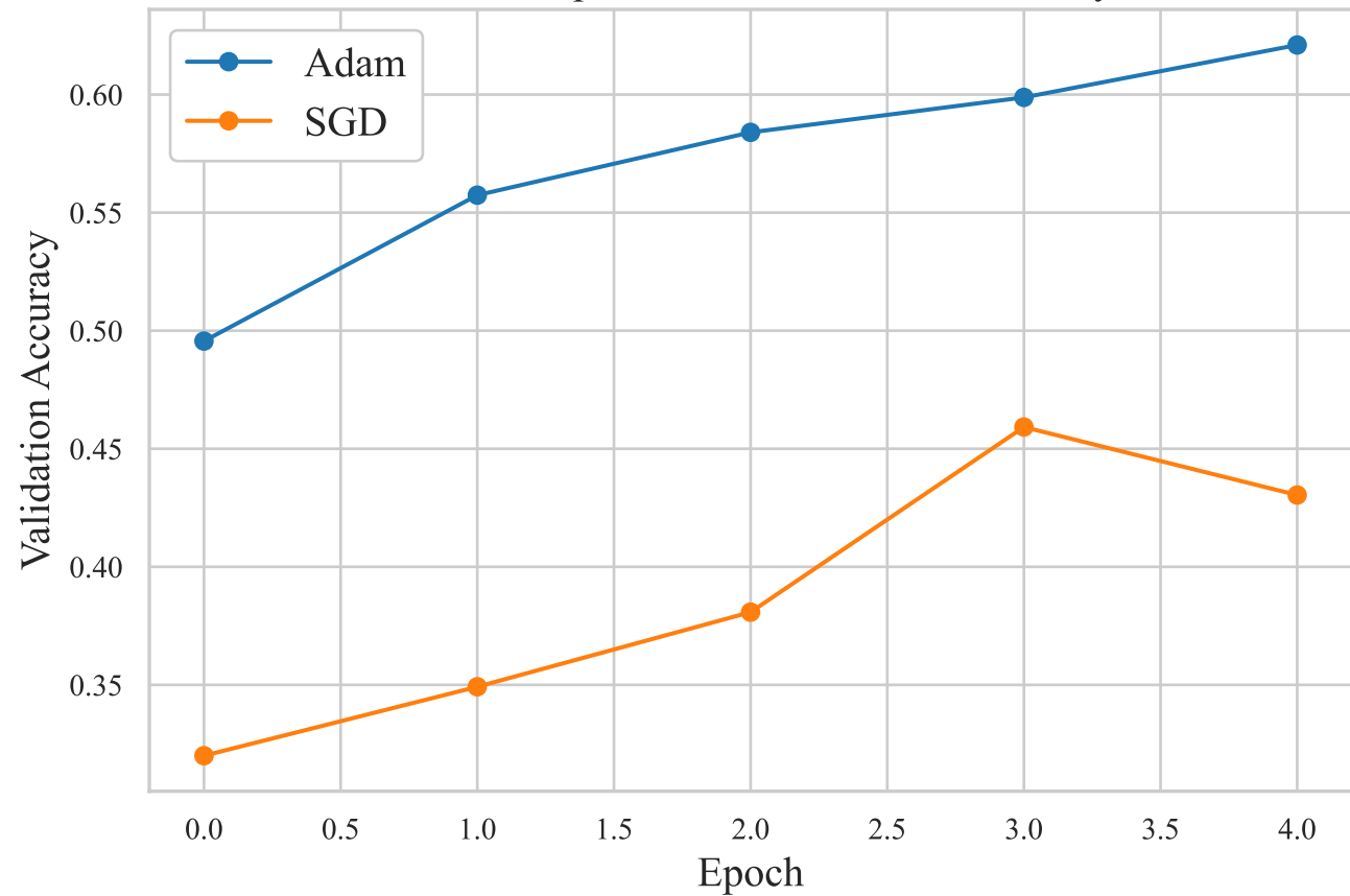
Effect of Optimizer on Validation Accuracy
